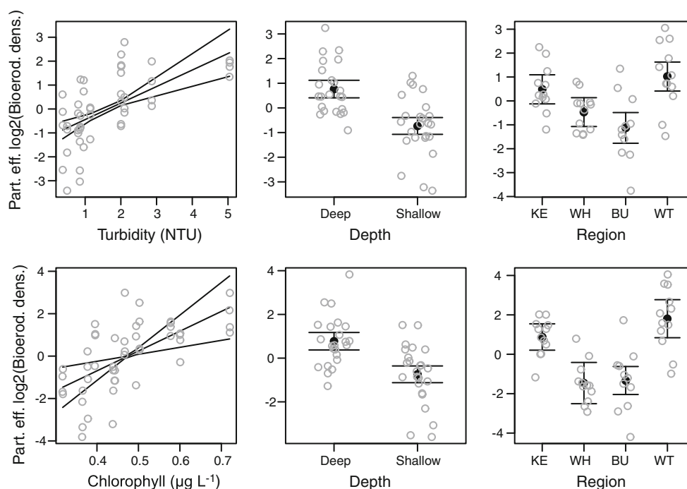
Fig. 5 Variation in bioeroders densities ( \log_2 -transformed) in inshore regions. The plots show outputs of partial dependence model response to changing turbidity (NTU) or chlorophyll ( \mu\text{g L}^{-1} ), across estimates of means and 95% CI, white points are residuals the 2 depth categories (deep and shallow) and the 4 Great Barrier Reef
