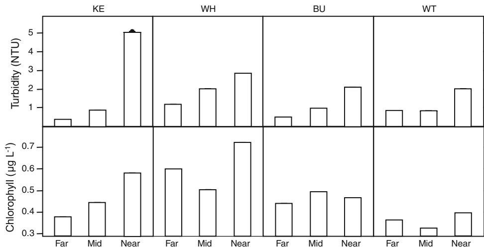
Fig. 3 Mean water column turbidity (NTU) and chlorophyll (µg L -1 ) at each station (near, mid, far from the river mouth) from the 4 Marine Monitoring Program regions of the Great Barrier Reef. KE Keppels, WH Whitsundays, BU Burdekin and WT Wet tropics. Data provided by the Reef Plan
